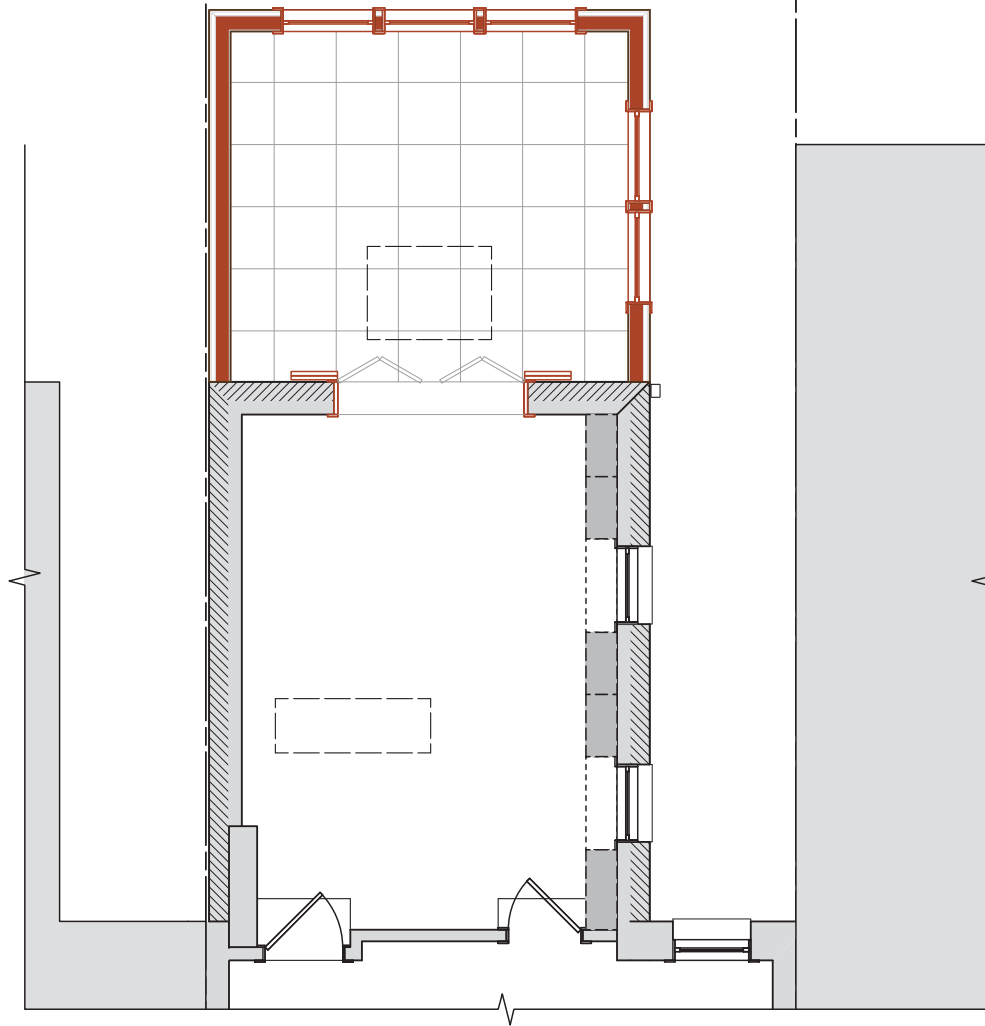
C Second Floor Plan (partial) 1/4" = 1'-0"
