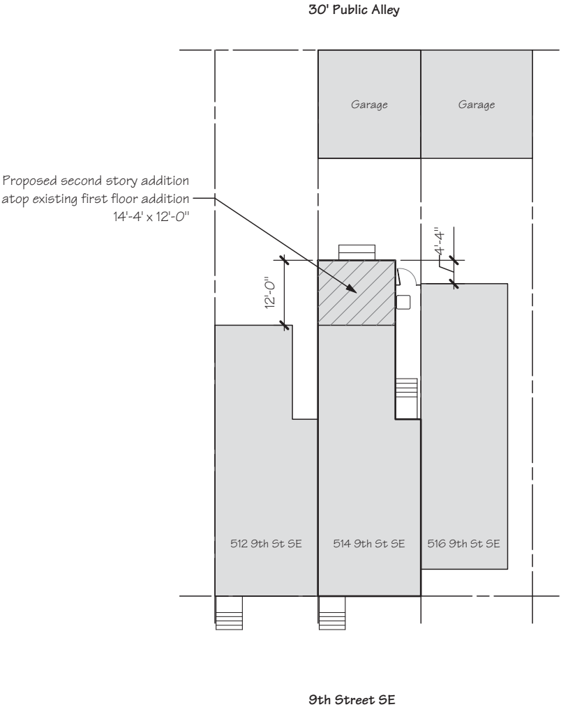
A Site Plan 1/16" = 1'-0"
